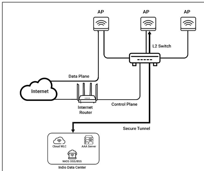
Figure 2. Indio access point with Indio's WiOS cloud controller.
